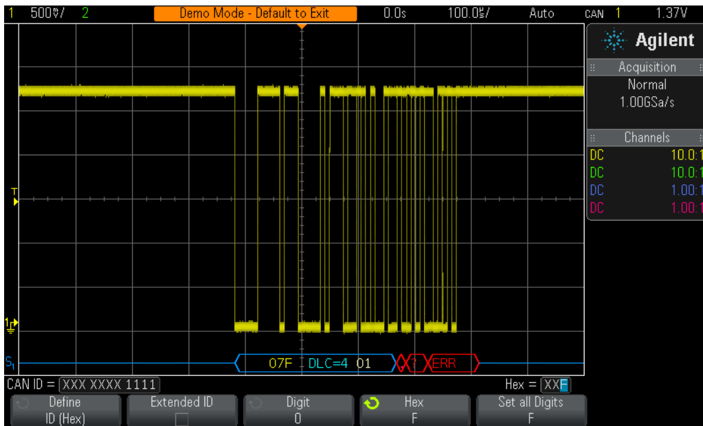
Figure 69 While triggering on CAN data frame = 07F_{\text{HEX}} , the scope’s hardware-based decoding reveals infrequent error conditions.
